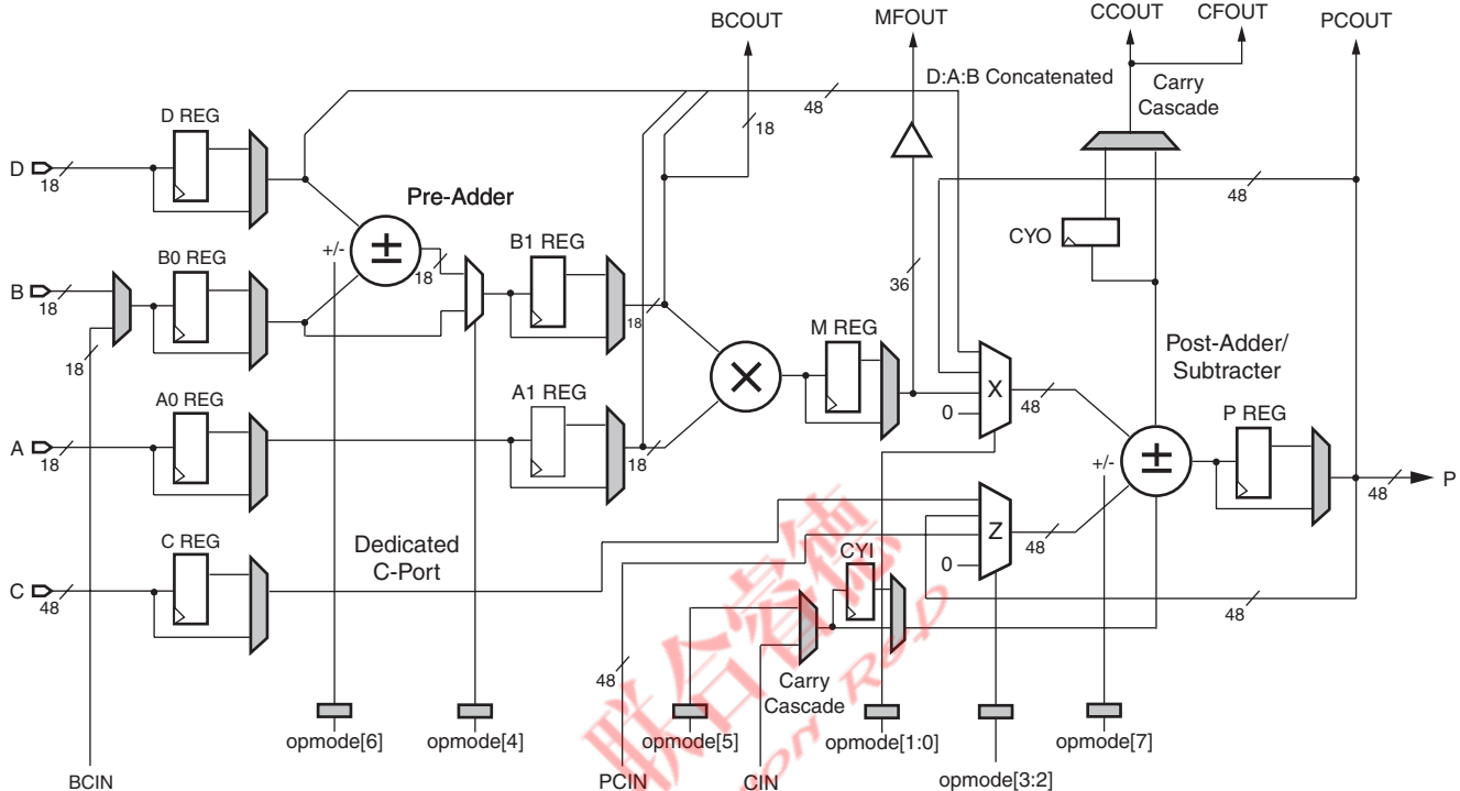
Figure 1-3: DSP48A1 Slice
