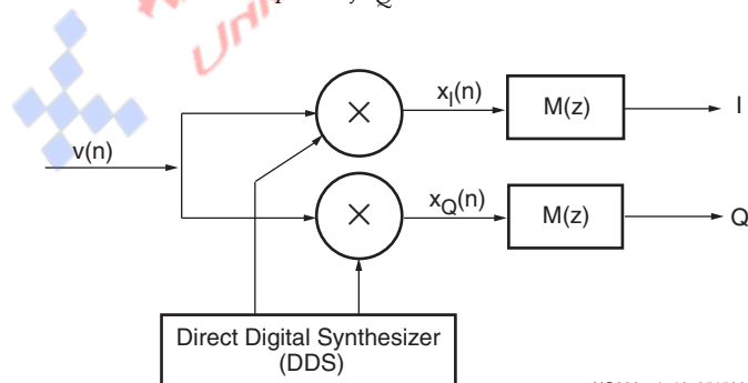
Figure 1-13: Software-Defined Radio Digital Down Converter
