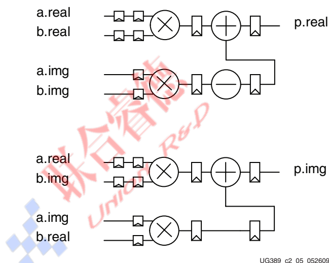
Figure 2-5: Four-Multiplier Complex Version
