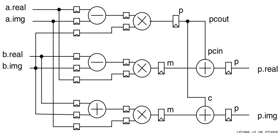
Figure 2-6: Three-Multiplier Complex Version
